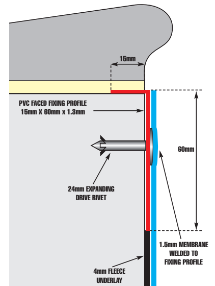
Side-Mount PVC Profile
