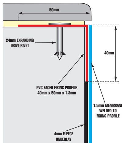
Top-Mount PVC Profile
